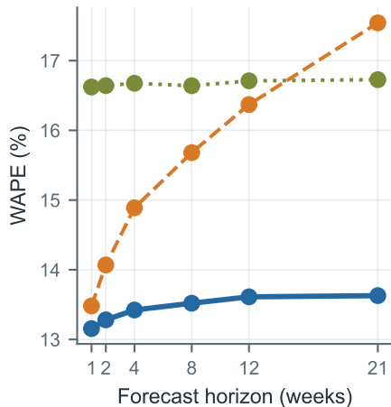
A. Cumulative forecast error
