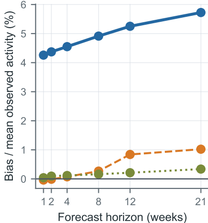
B. Normalised prediction bias
